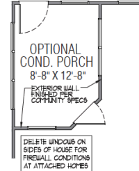
OPT. COND. PORCH
