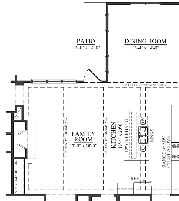
"OPTIONAL" FAMILY ROOM w/ BEAMS & LARGER DINING ROOM
