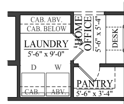
"OPTIONAL" LAUNDRY / PANTRY / HOME OFFICE
